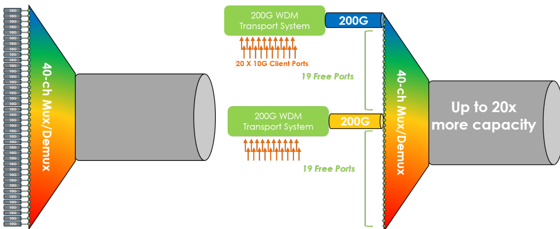
Figure 8a & 8b - Reclaiming capacity on an existing WDM system using alien wavelengths
