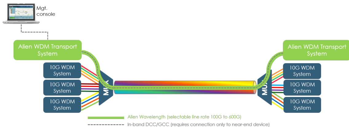
Figure 7 - Alien wavelength deployment
